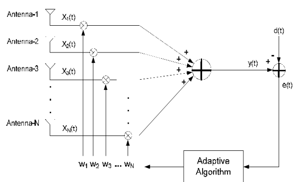
Fig.1. Adaptive beam-forming block diagram is generally the best choice for many different applications of adaptive signal processing.
